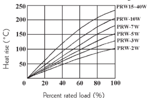
Derating curve:
